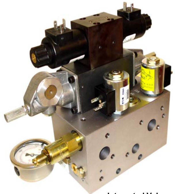
Integrated Valve
